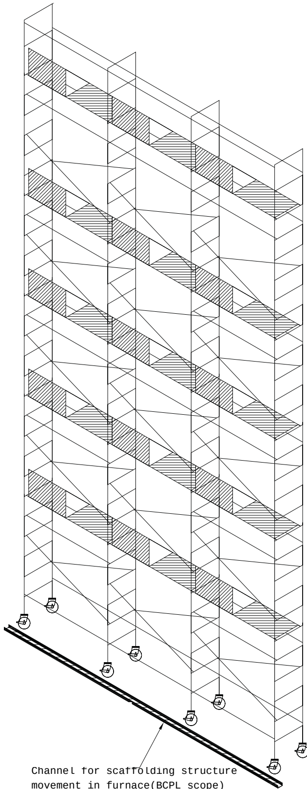
Conceptual Drawing for Aluminium Scaffolding system inside Furnace
